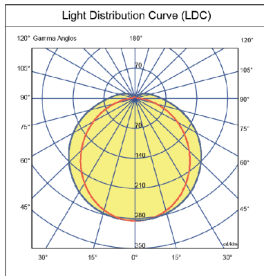
WPUT220-R85
