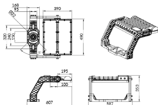
FLZ 600W-800W(without driver)
