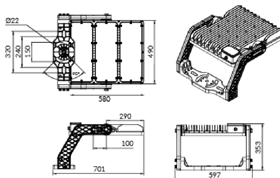
FLZ 1000W-1200W(without driver)
