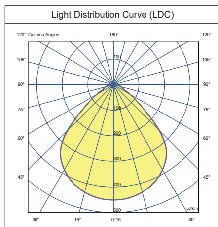
FPUW235W4K-C
