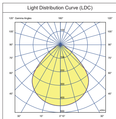
FPUW235W4K-Z
