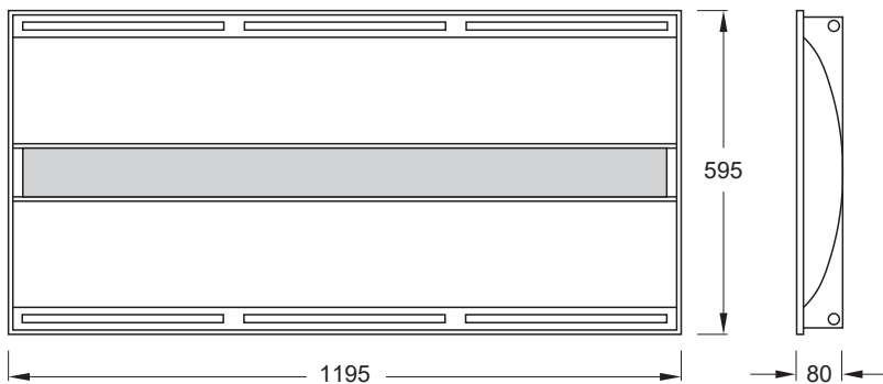
NUDW4 (Air Handling) - 1200x600 mm
