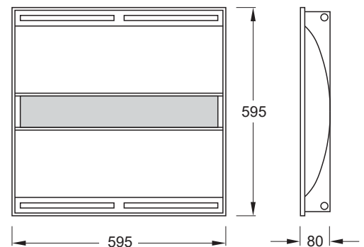
NUDW2 (Air Handling) - 600x600 mm
