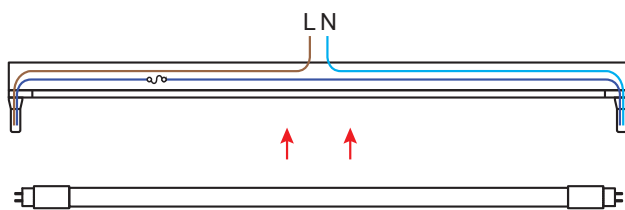
Type A LED lamp
