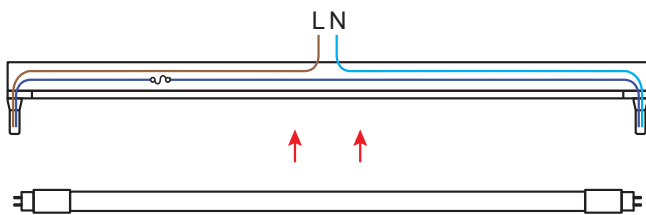
Type A LED lamp
