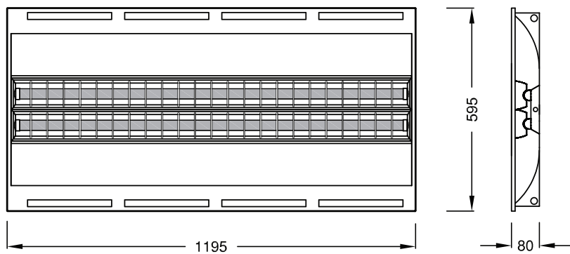
NULW4 (Air Handling) - 1200x600 mm
