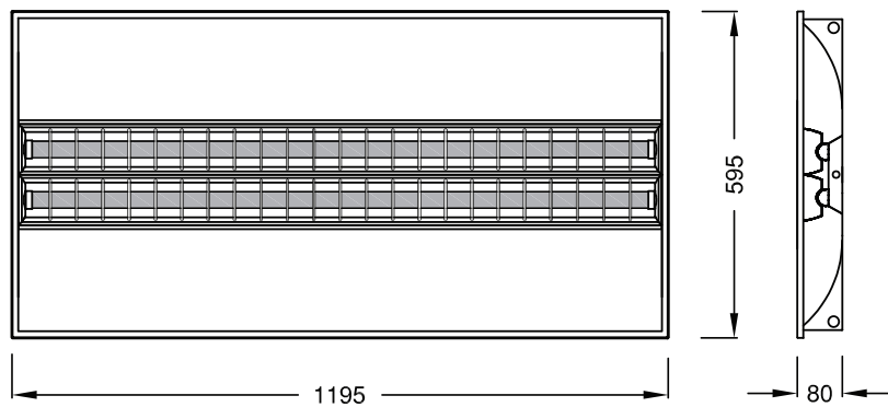
NULW4 - 1200x600 mm
