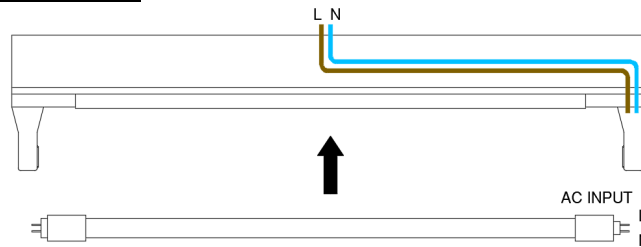
Type B LED Lamp
